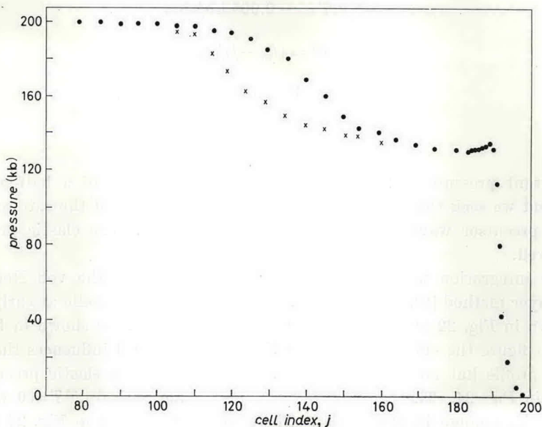
Fig. 23. - Double shock in iron. (Ref. [9]). p_1 = 0.200 Mb; cell width = 0.01 cm; \bullet \Delta V = -0.004 \text{cm}^3/\text{g} ; \times \Delta V = -0.0059 \text{cm}^3/\text{g} ; \tau = \frac{1}{3} \mu s.
